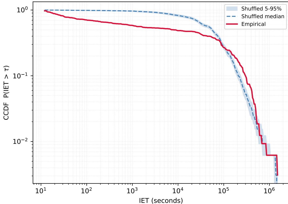
User 302926911 - Empirical vs Reshuffled | KS=0.403 p=0.000
